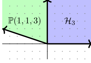
FIGURE 3. The secondary fan of the Hirzebruch surface \mathcal{H}_3 , which has two chambers; (blue) corresponding to \mathcal{H}_3 and (green) corresponding to \mathbb{P}(1,1,3) .
